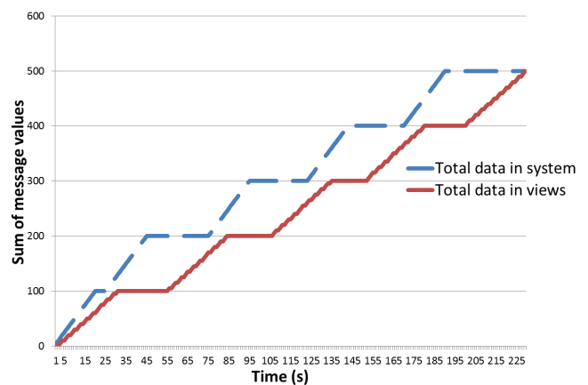
Fig. 5 Normal progress of the active Lambda architecture implementation.
