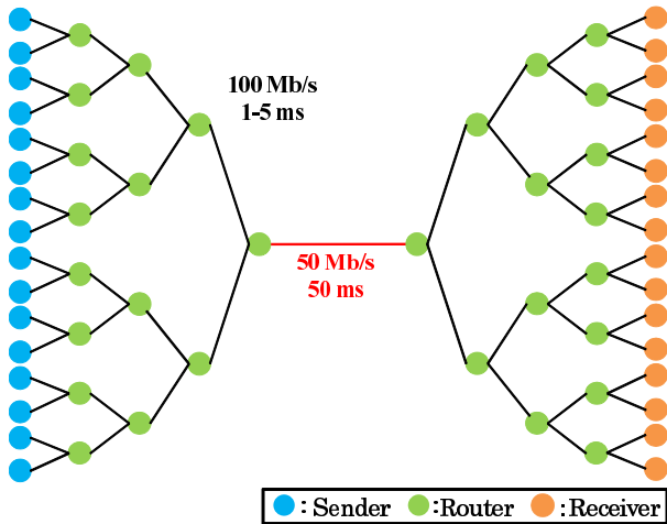
Fig. 5 Simulation model.
