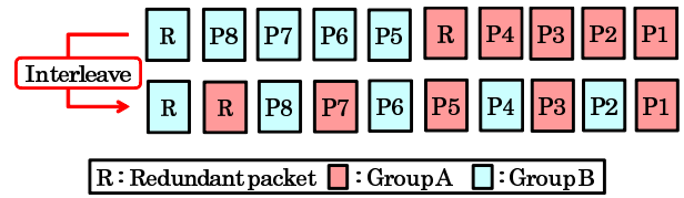
Fig. 3 Interleave control.
