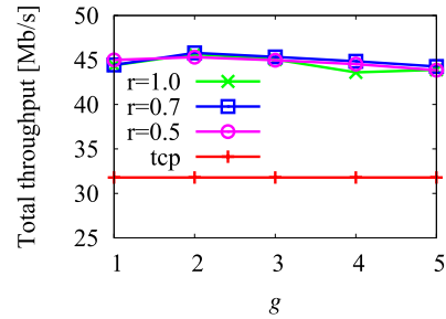
(a) Total throughput
