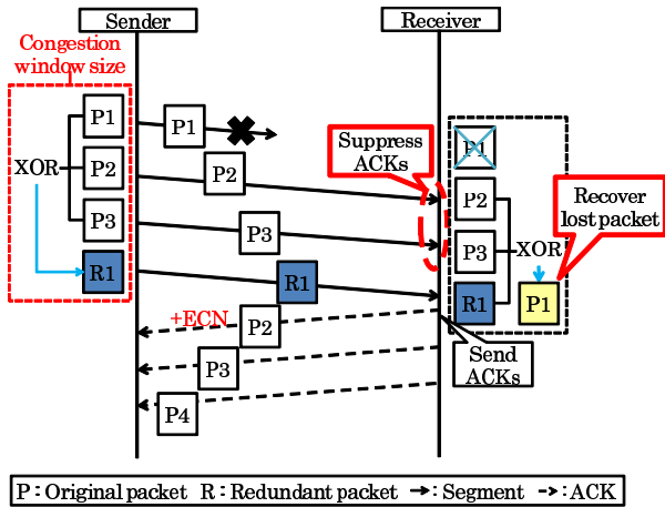
Fig. 2 Proposed scheme.
