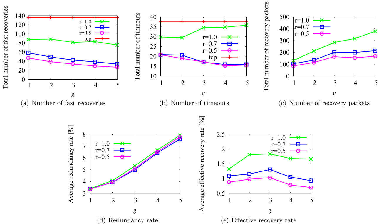
Fig. 7 Analysis of the characteristics (0–60 s).
