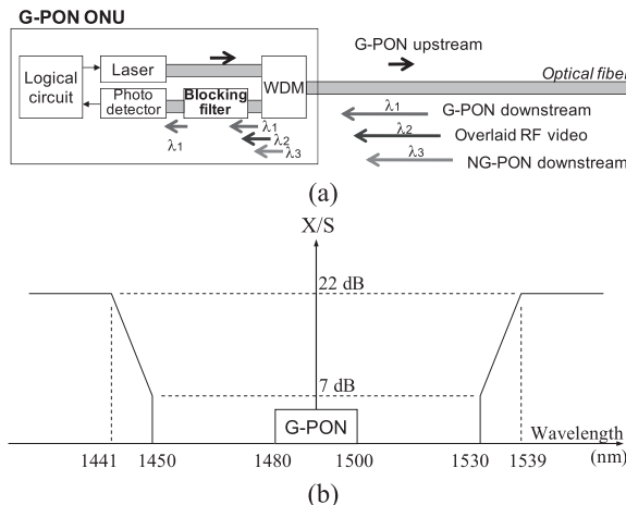
Fig. 2 (a) G-PON ONU employing the blocking filter, and (b) characteristic of the blocking filter as defined in G.984.5.
