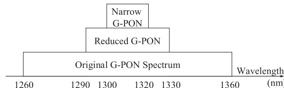
Fig. 3 The ONU spectrum plan options as defined in G.984.5.
