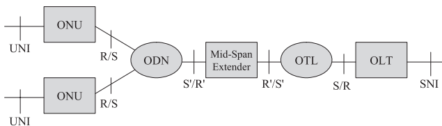
Fig. 5 A mid-span reach extended PON.
