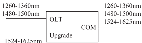
Fig. 4 The WDM1 filter defined in G.984.5.
