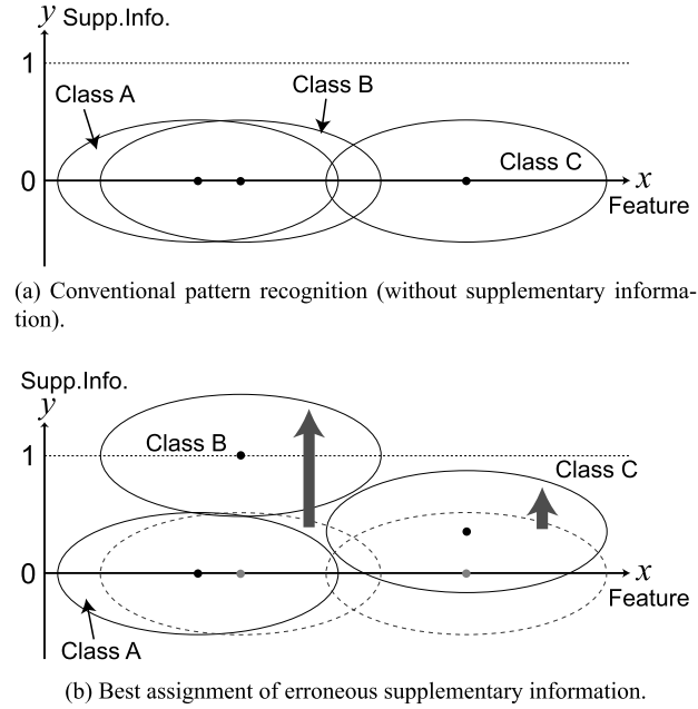
Fig. 13 Class distributions and assignment of erroneous supplementary information. Ellipses represent equiprobable lines of class distributions.
