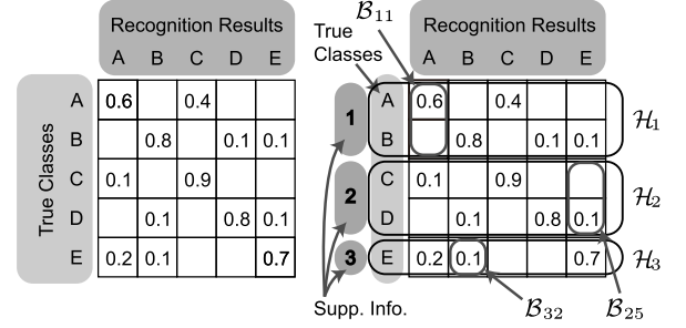
(a) A confusion matrix in prob- (b) Assignment of symbols that achieves a 100% recognition rate.
