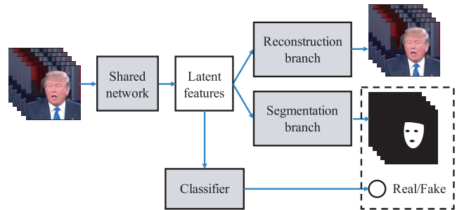
Fig. 5 Overview of the multitask network [67].
